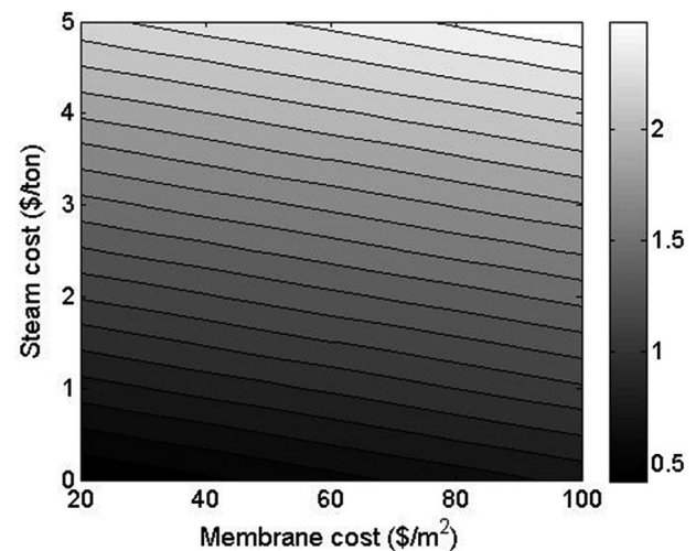
Fig. 7. Contours of water cost ($/m 3 ) of MD system at different membrane and steam cost.
