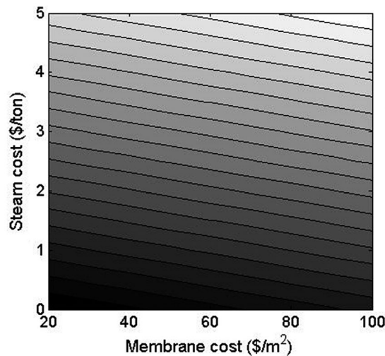
Fig. 16. Contours of water cost ($/m 3 ) of RO-MD hybrid system at different membrane cost and steam cost.
